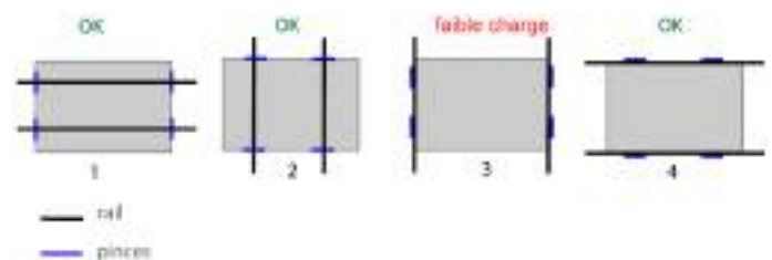
Figure 3: Configurations de montage
