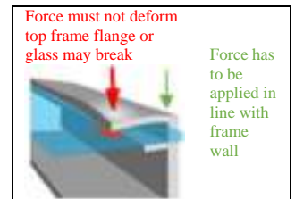
Figure 1a: Clamp Force Locations
